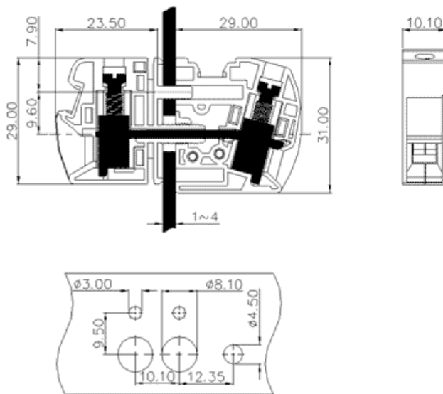
钻孔图 For a drilling diagram
